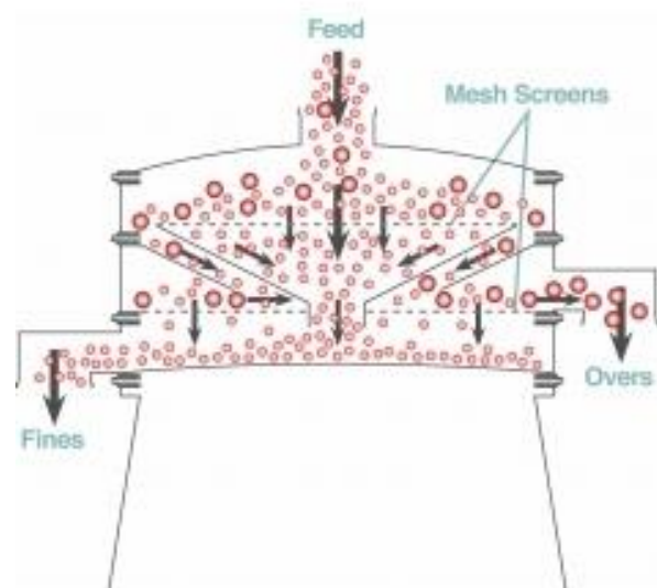
Fig. 2: RJ-VS-2200 Vibrating Sieve
